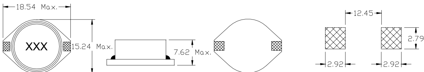
TOP VIEW
